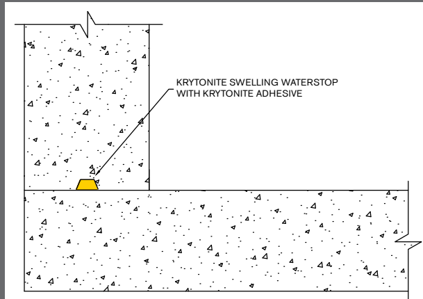
WALL TO SLAB OR WALL TO ELEVATED SLAB CONSTRUCTION JOINTS
