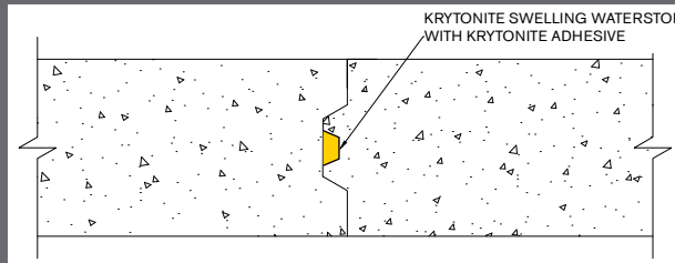
SLAB TO SLAB OR WALL TO WALL CONSTRUCTION JOINTS
