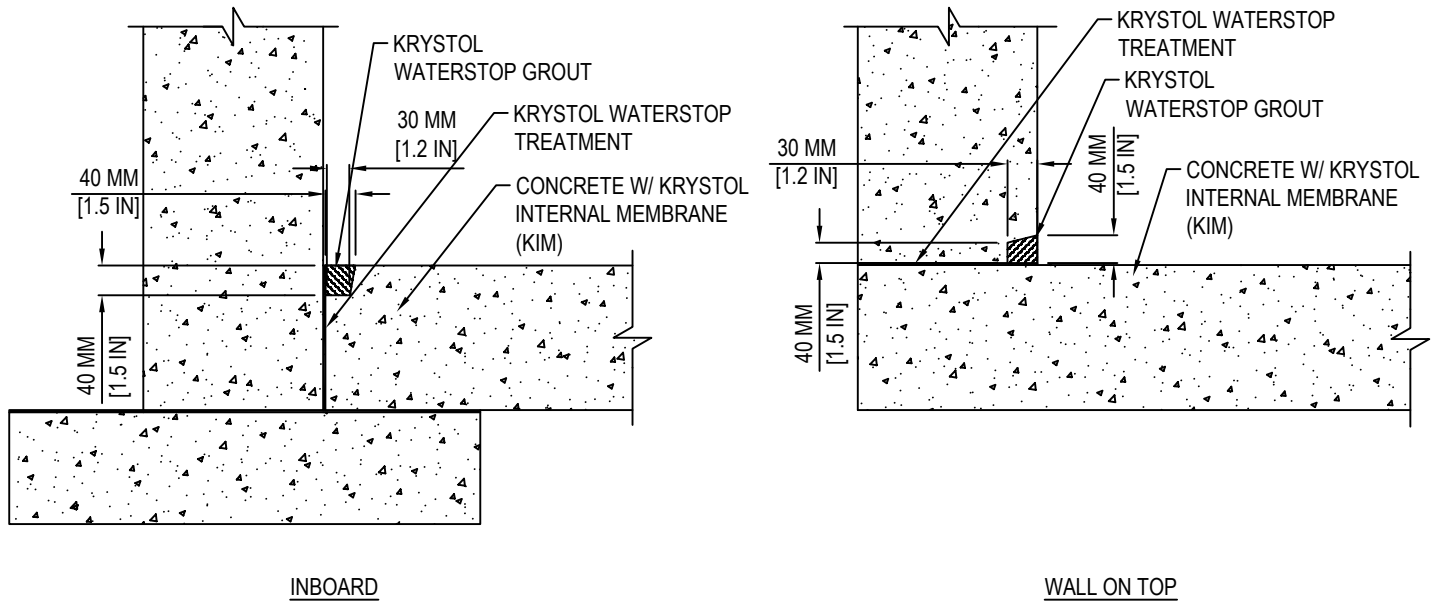
WALL TO SLAB CONSTRUCTION JOINTS DUAL PROTECTION; EXTERNAL GROUT METHOD
