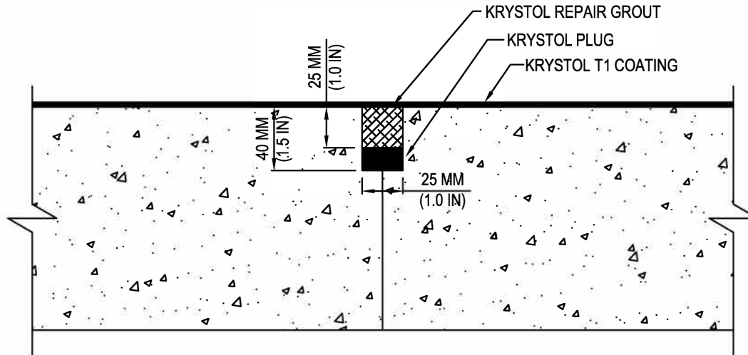
SLAB TO SLAB/WALL TO WALL JOINT REPAIR
