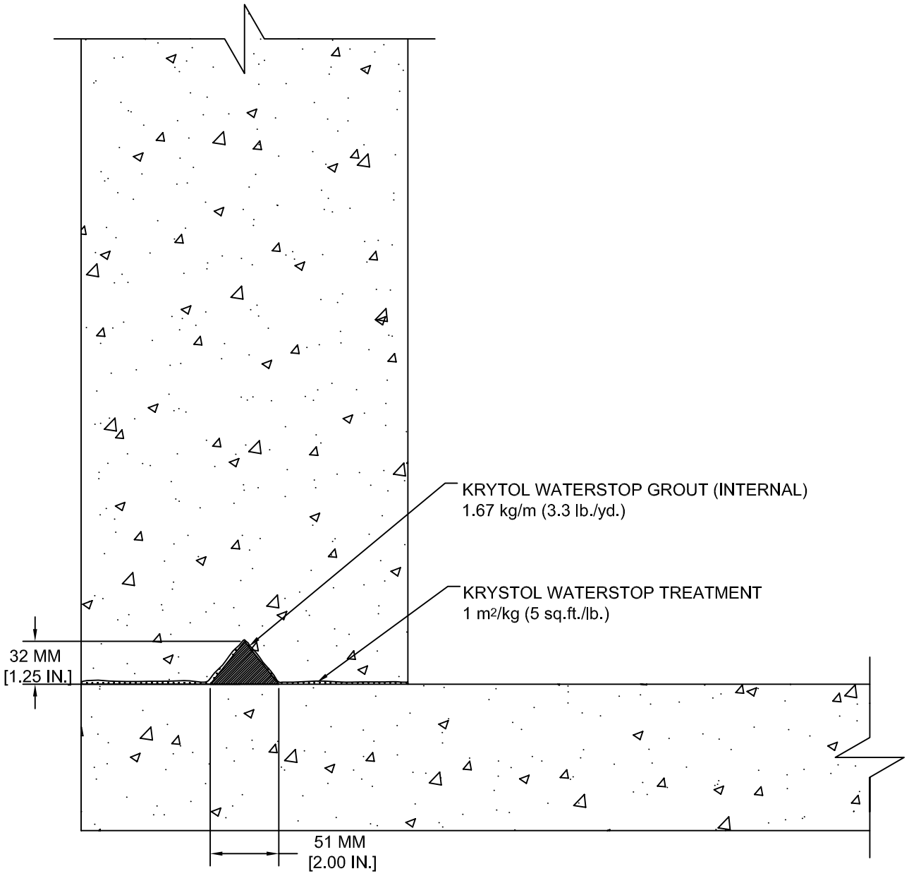
NEW CONSTRUCTION - WALL TO SLAB - SHOTCRETE (WALL ON TOP OF SLAB)
