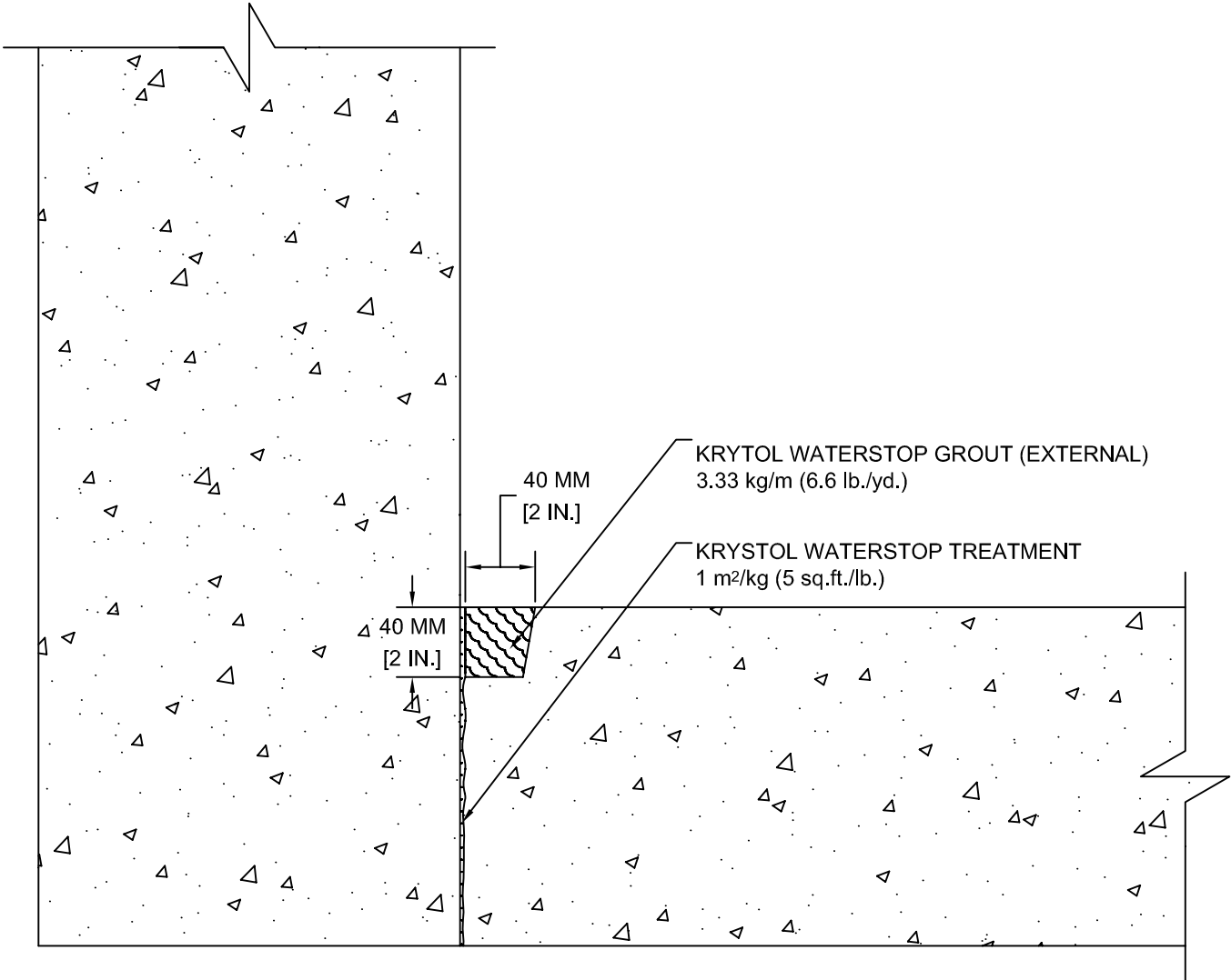
NEW CONSTRUCTION - WALL TO SLAB - SHOTCRETE (WALL INBOARD OF SLAB)
