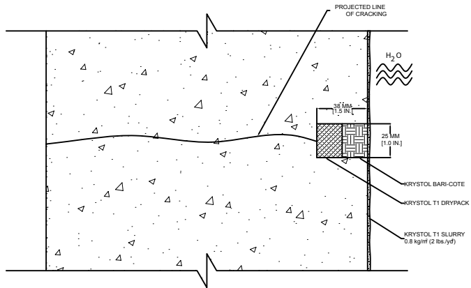
POSITIVE SIDE CRACK REPAIR (CROSS SECTION)
