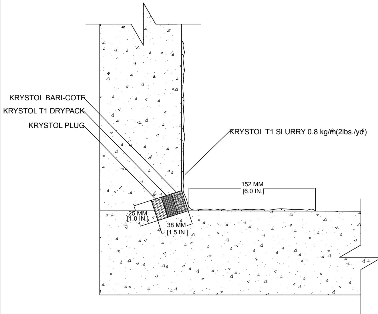
JOINT REPAIR - WALL TO SLAB (WALL ON TOP OF SLAB)
