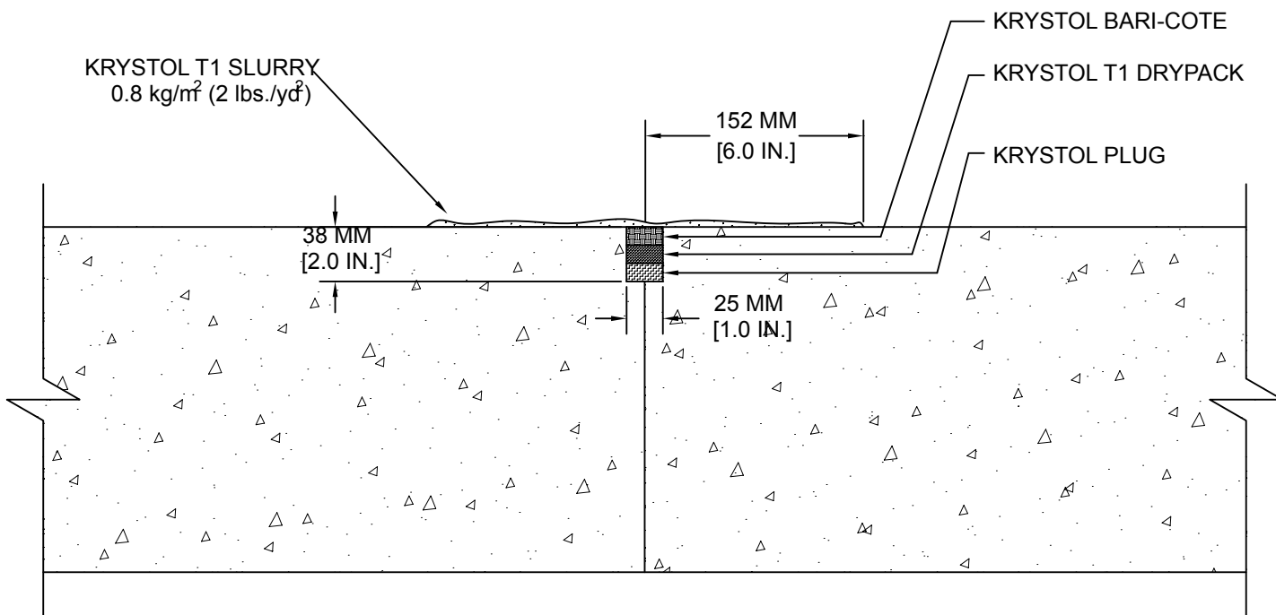
CRACK OR JOINT REPAIR - SLAB TO SLAB
