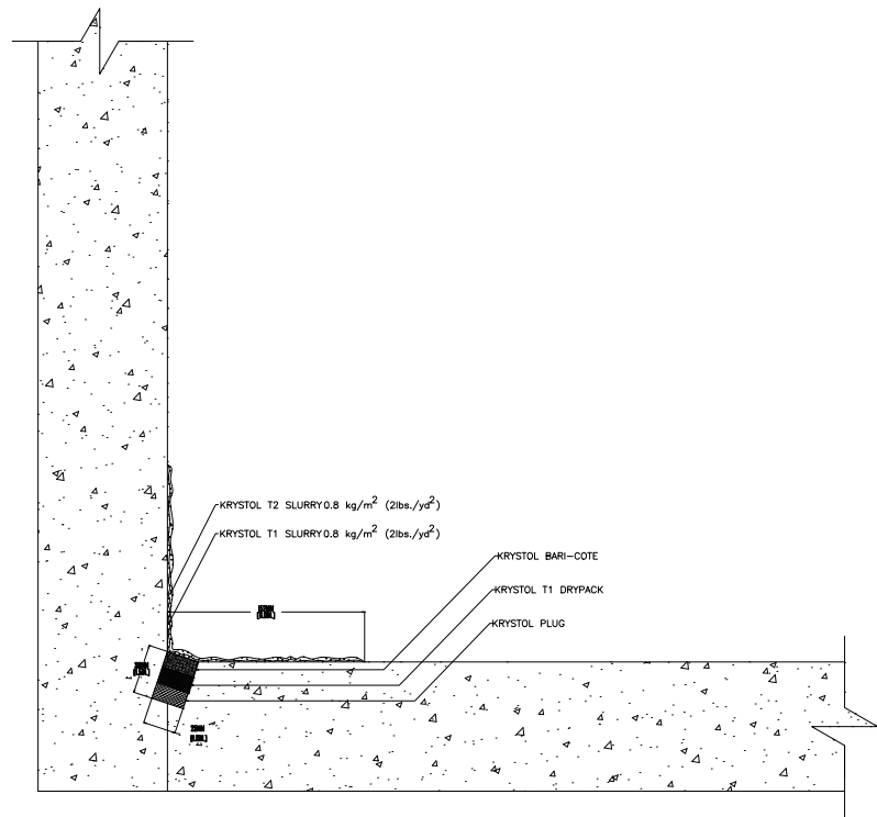
JOINT REPAIR – WALL TO SLAB (INBOARD)
