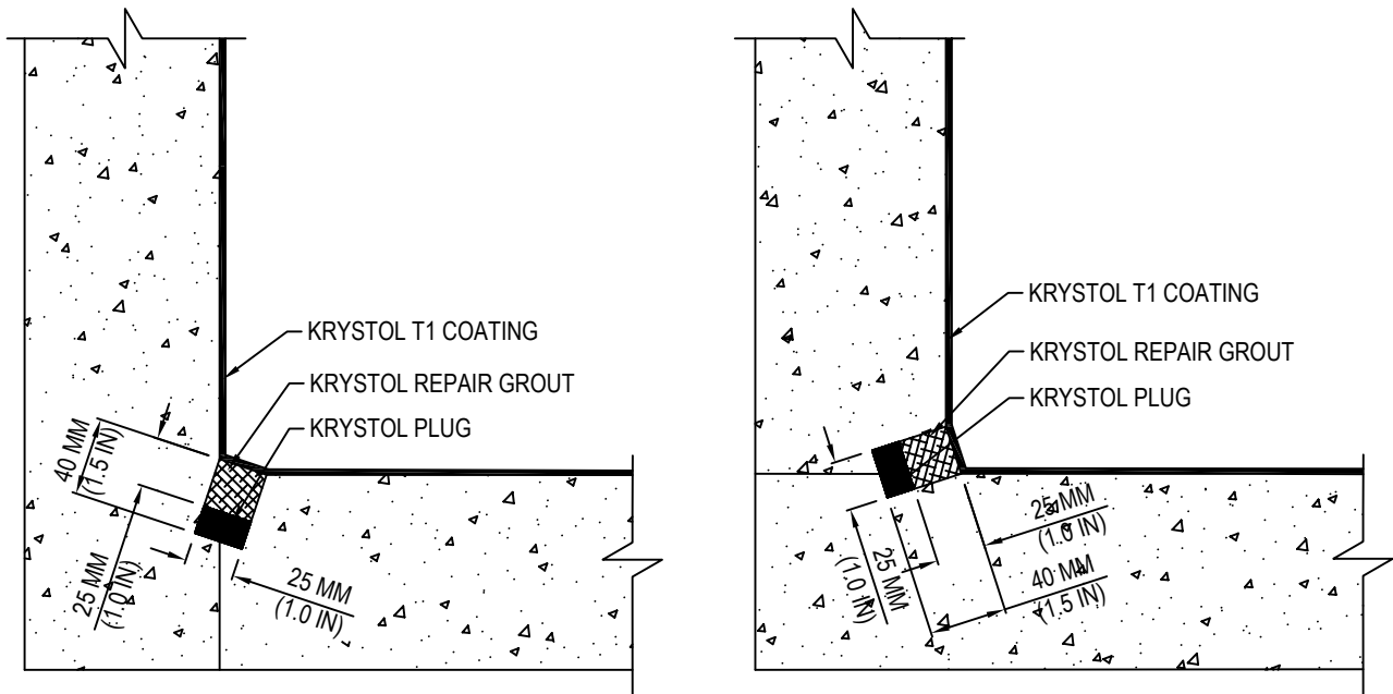
WALL TO SLAB JOINT REPAIR
